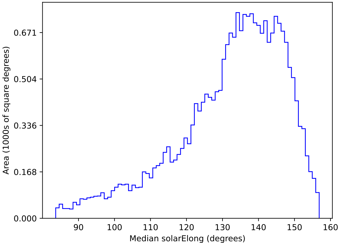
too_elab_r32_d2_giz_v3.4_10yrs All sky u band: Median solarElong
