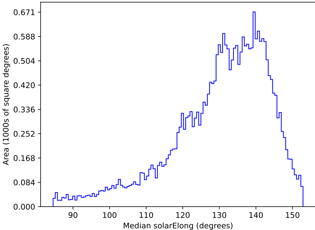
too_elab_r32_d2_giz_v3.4_10yrs All sky r band: Median solarElong
