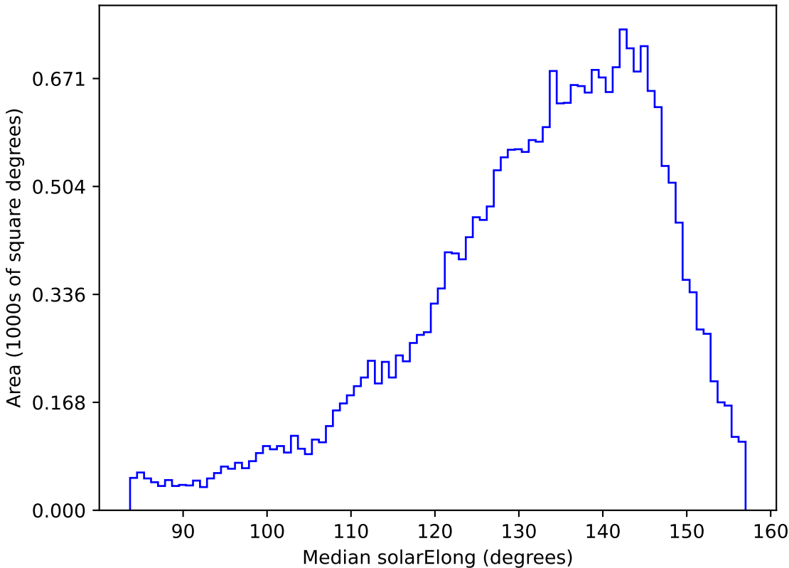
too_elab_r32_d2_giz_v3.4_10yrs All sky g band: Median solarElong
