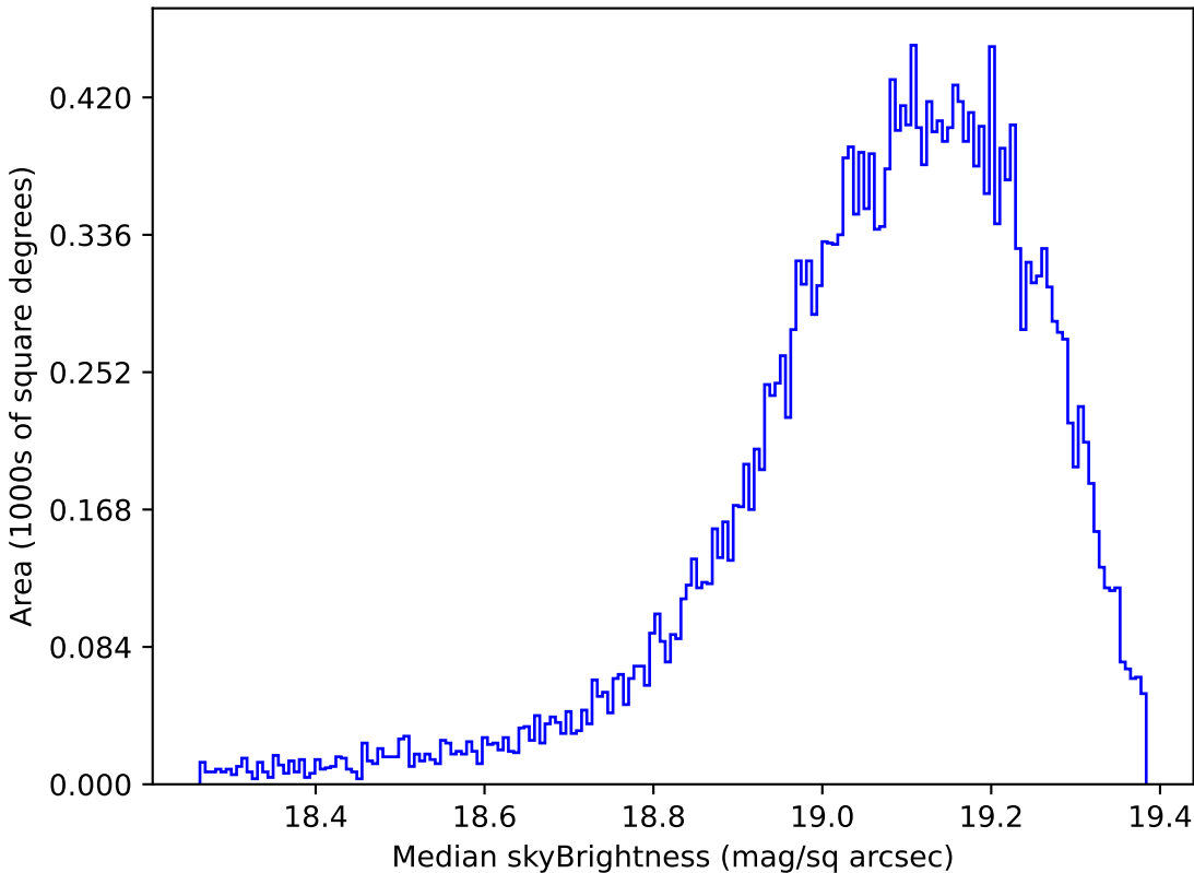
too_elab_r32_d2_giz_v3.4_10yrs Yr 1 z band: Median skyBrightness
