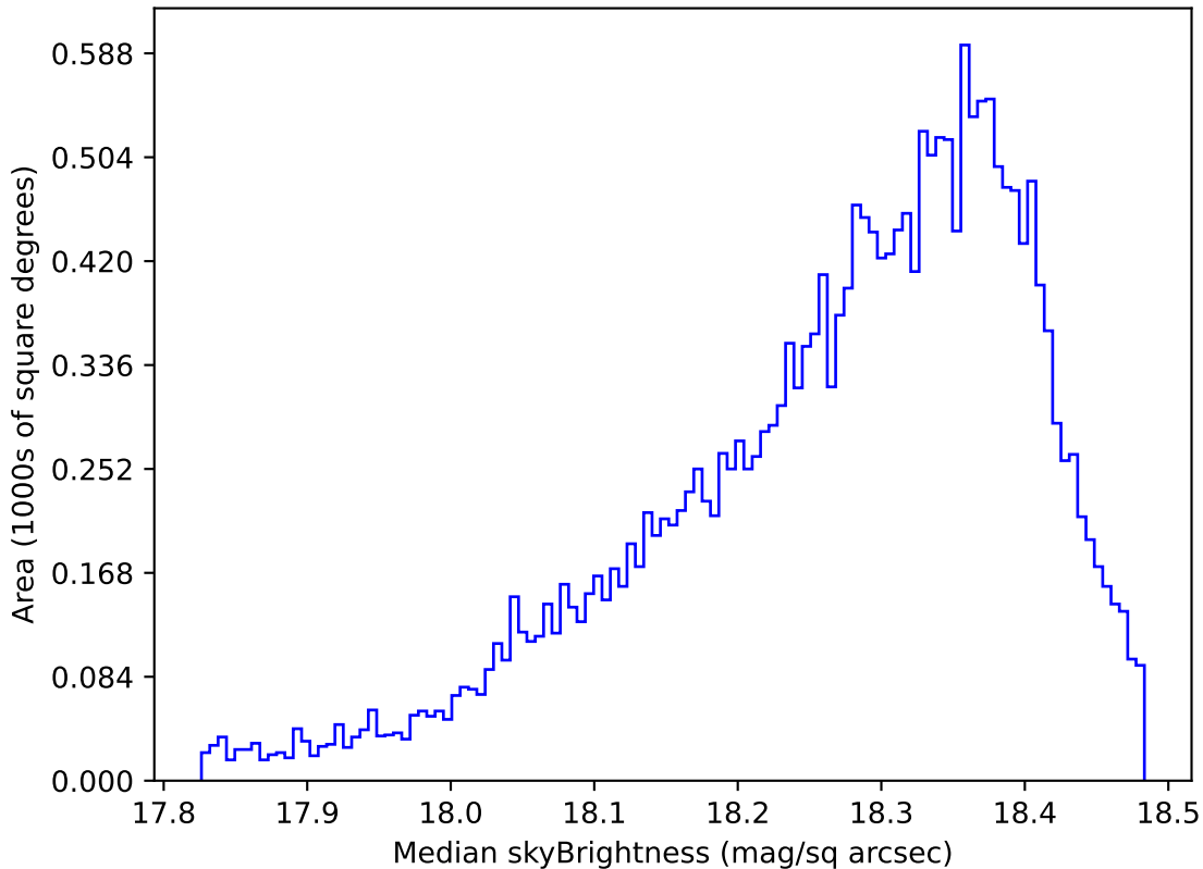
too_elab_r32_d2_giz_v3.4_10yrs Yr 1 y band: Median skyBrightness
