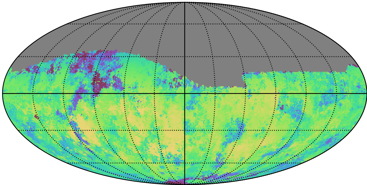
too_elab_r32_d2_giz_v3.4_10yrs Yr 1 i band: Median skyBrightness
