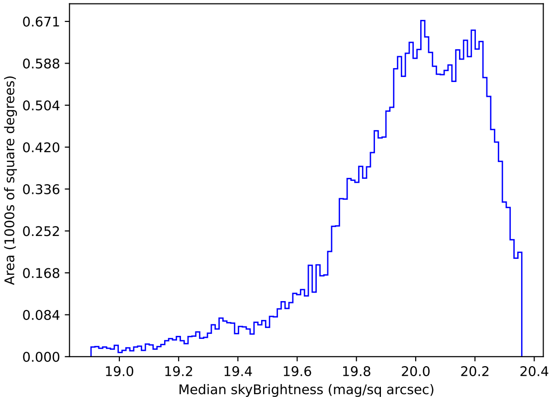
too_elab_r32_d2_giz_v3.4_10yrs Yr 1 i band: Median skyBrightness
