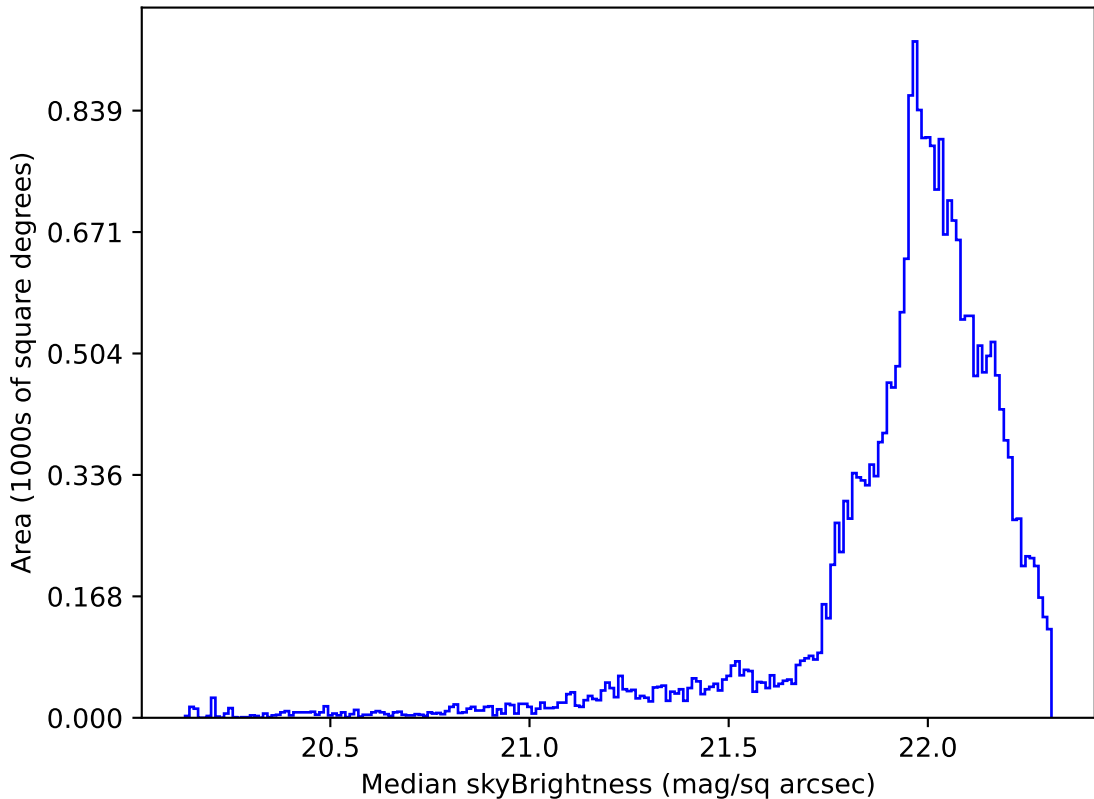
too_elab_r32_d2_giz_v3.4_10yrs Yr 1 g band: Median skyBrightness
