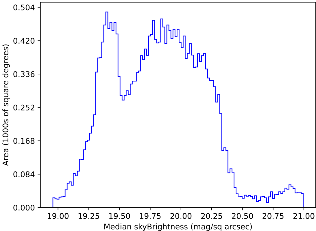
too_elab_r32_d2_giz_v3.4_10yrs Yr 1 all bands: Median skyBrightness
