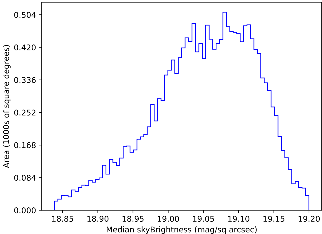
too_elab_r32_d2_giz_v3.4_10yrs WFD z band: Median skyBrightness
