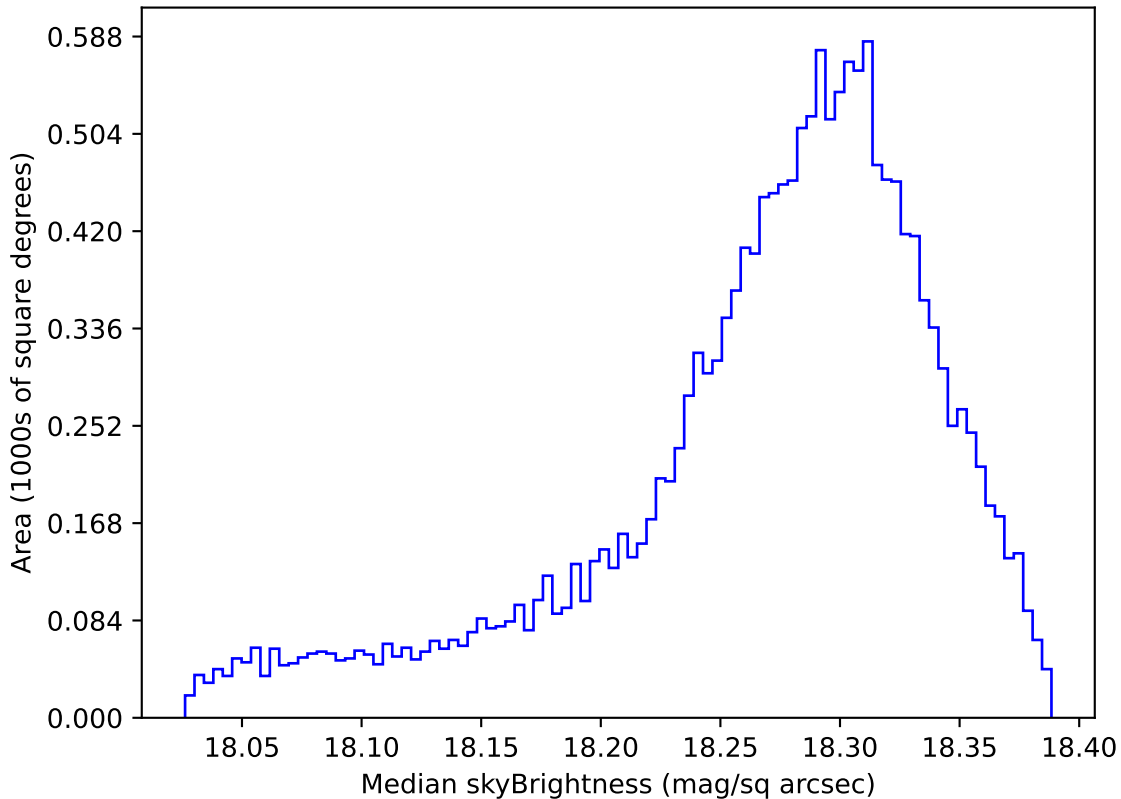
too_elab_r32_d2_giz_v3.4_10yrs WFD y band: Median skyBrightness
