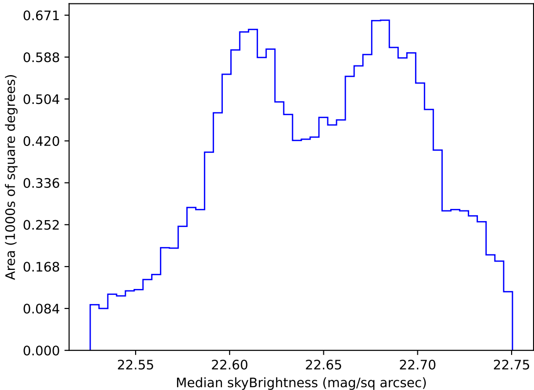
too_elab_r32_d2_giz_v3.4_10yrs WFD u band: Median skyBrightness
