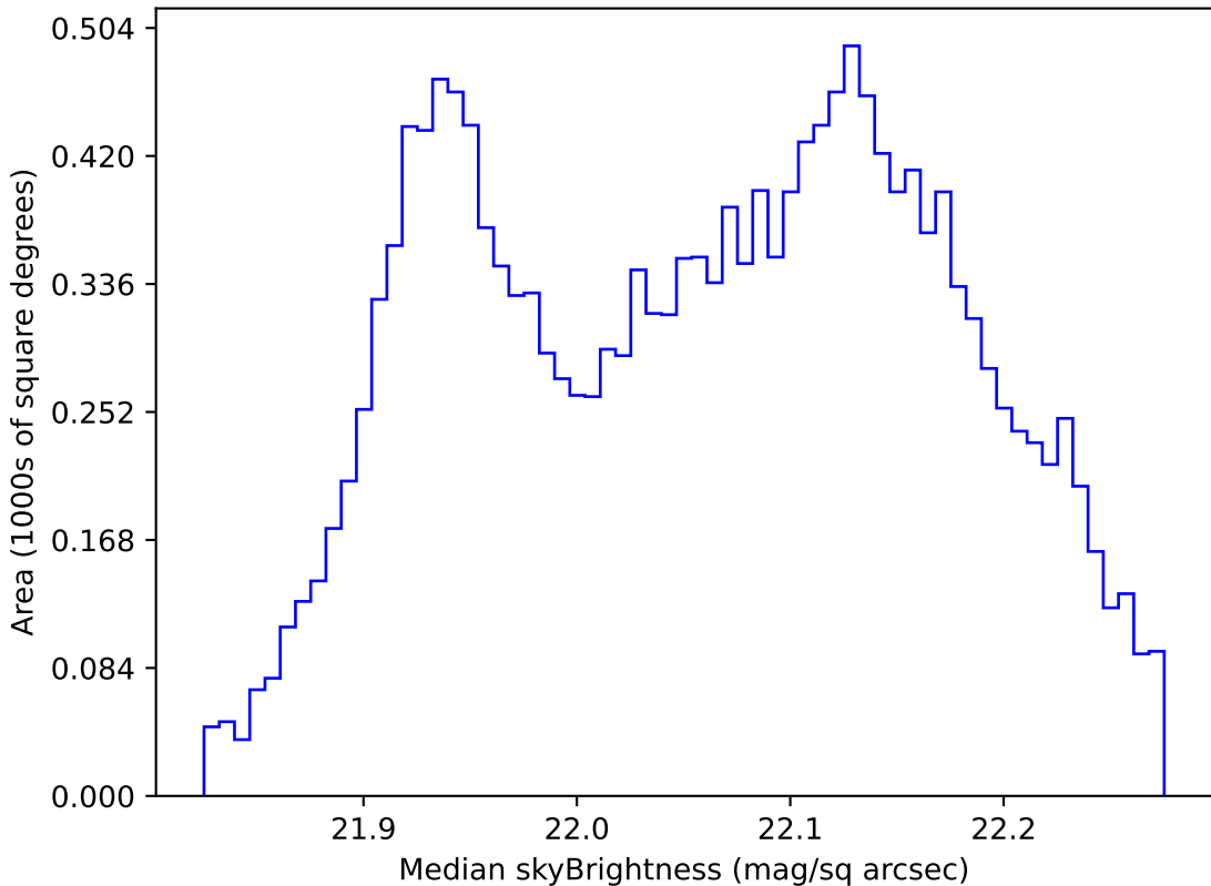
too_elab_r32_d2_giz_v3.4_10yrs WFD g band: Median skyBrightness
