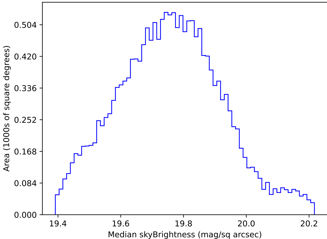
too_elab_r32_d2_giz_v3.4_10yrs WFD all bands: Median skyBrightness
