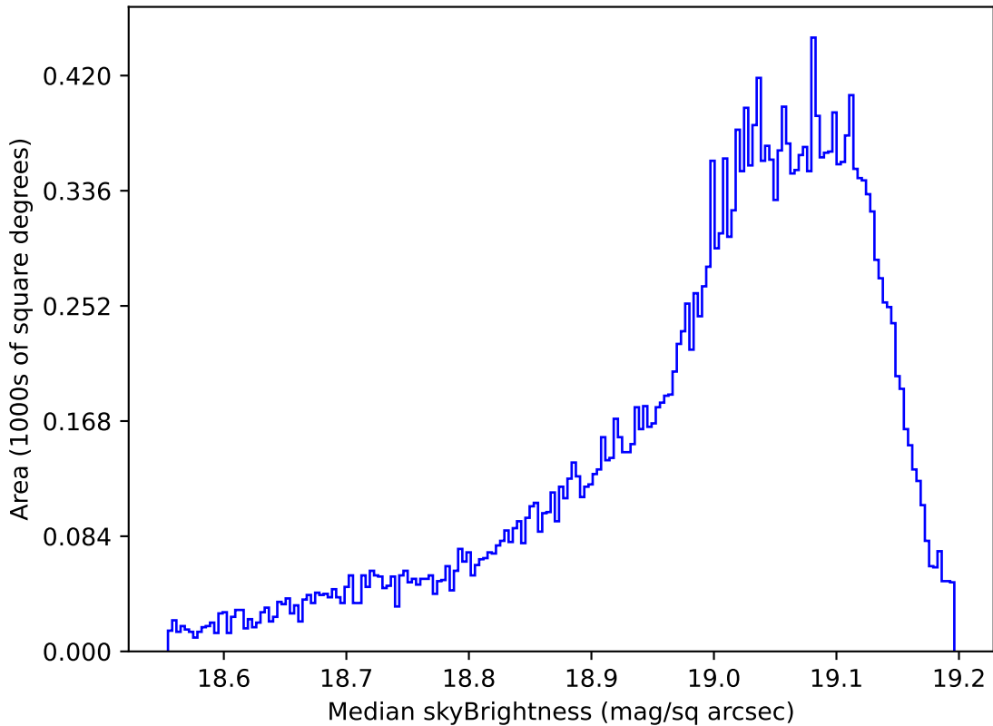
too_elab_r32_d2_giz_v3.4_10yrs All sky z band: Median skyBrightness
