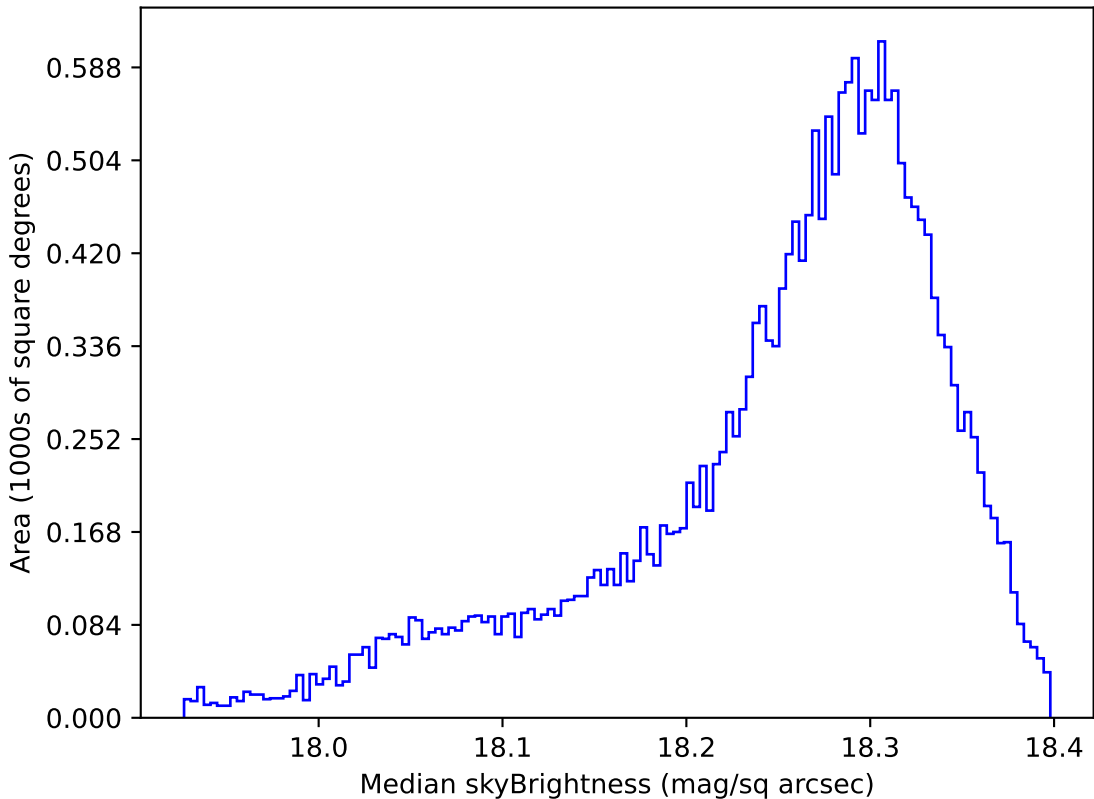
too_elab_r32_d2_giz_v3.4_10yrs All sky y band: Median skyBrightness
