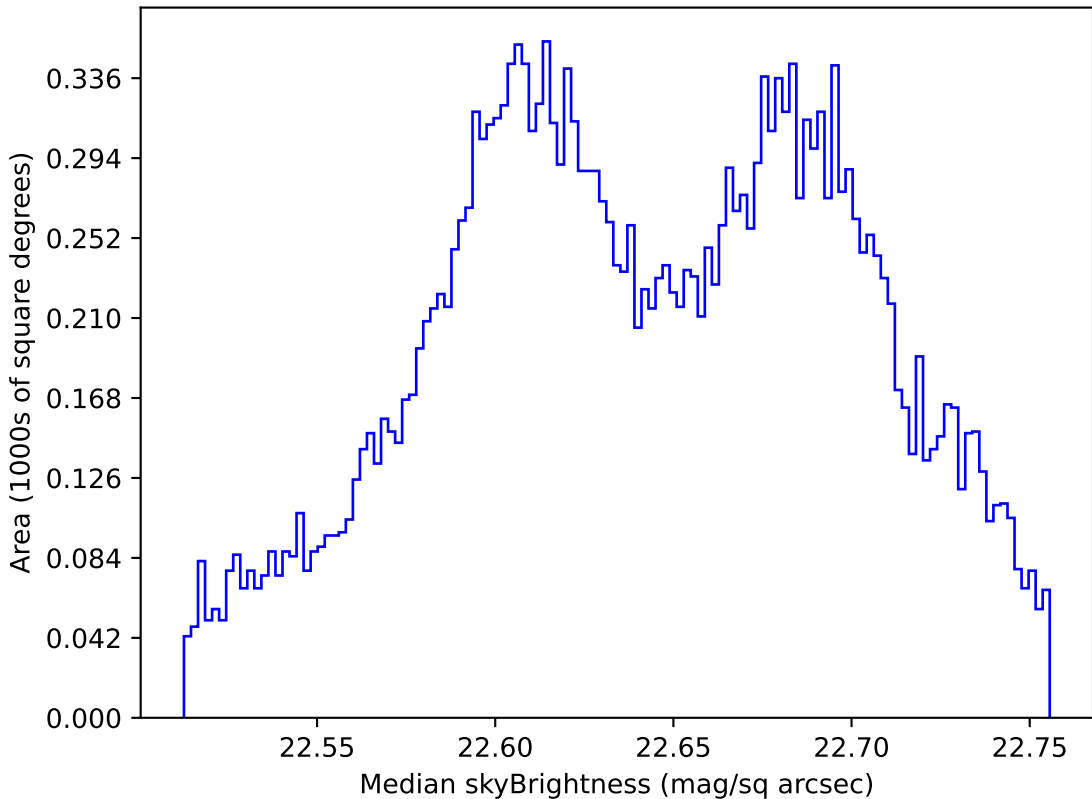
too_elab_r32_d2_giz_v3.4_10yrs All sky u band: Median skyBrightness
