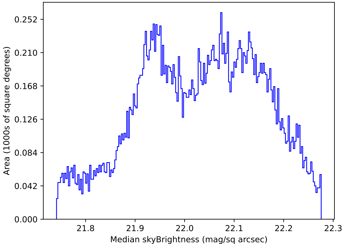
too_elab_r32_d2_giz_v3.4_10yrs All sky g band: Median skyBrightness
