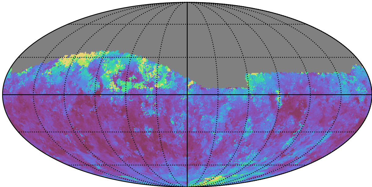
too_elab_r32_d2_giz_v3.4_10yrs Yr 1 z band: Median seeingEff
