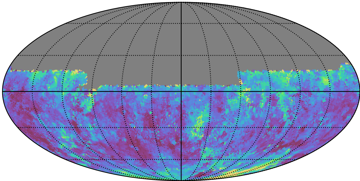
too_elab_r32_d2_giz_v3.4_10yrs Yr 1 y band: Median seeingEff
