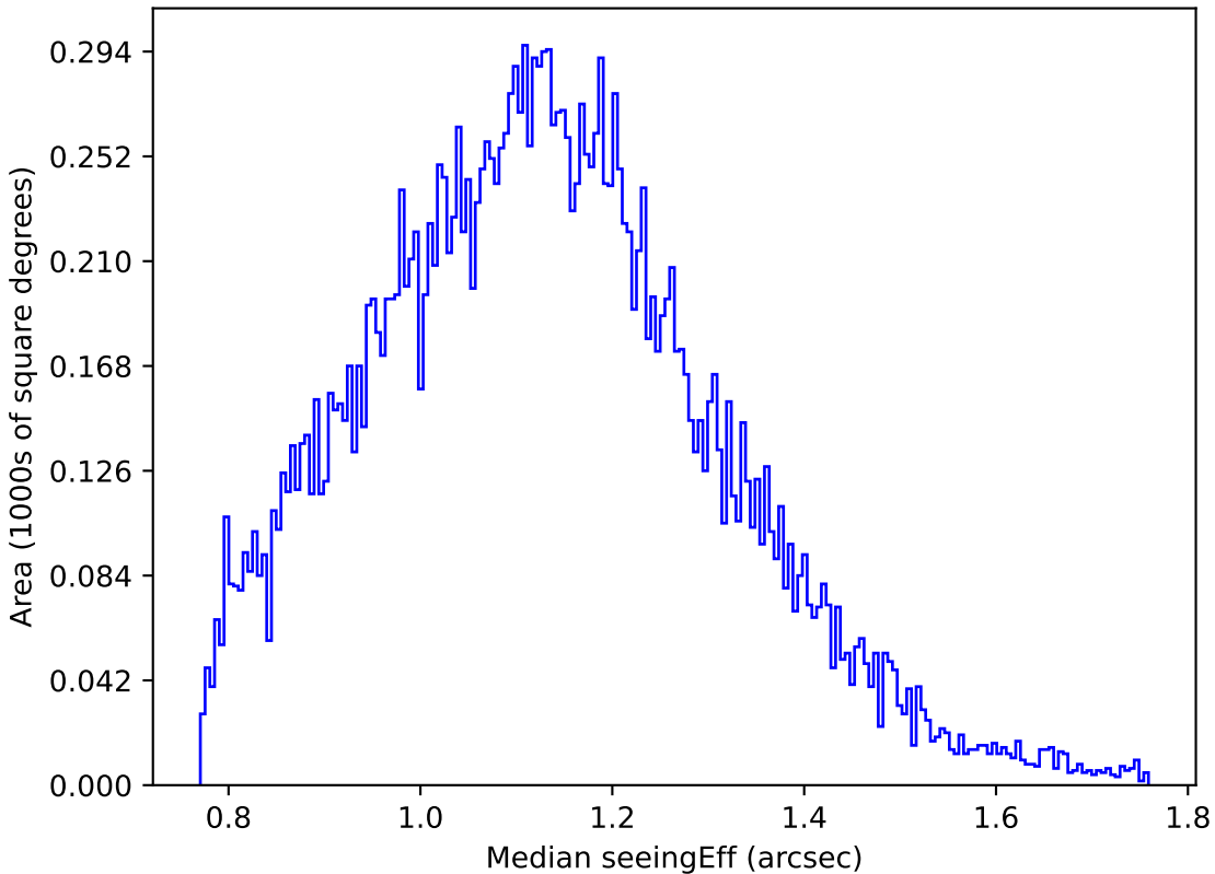
too_elab_r32_d2_giz_v3.4_10yrs Yr 1 u band: Median seeingEff
