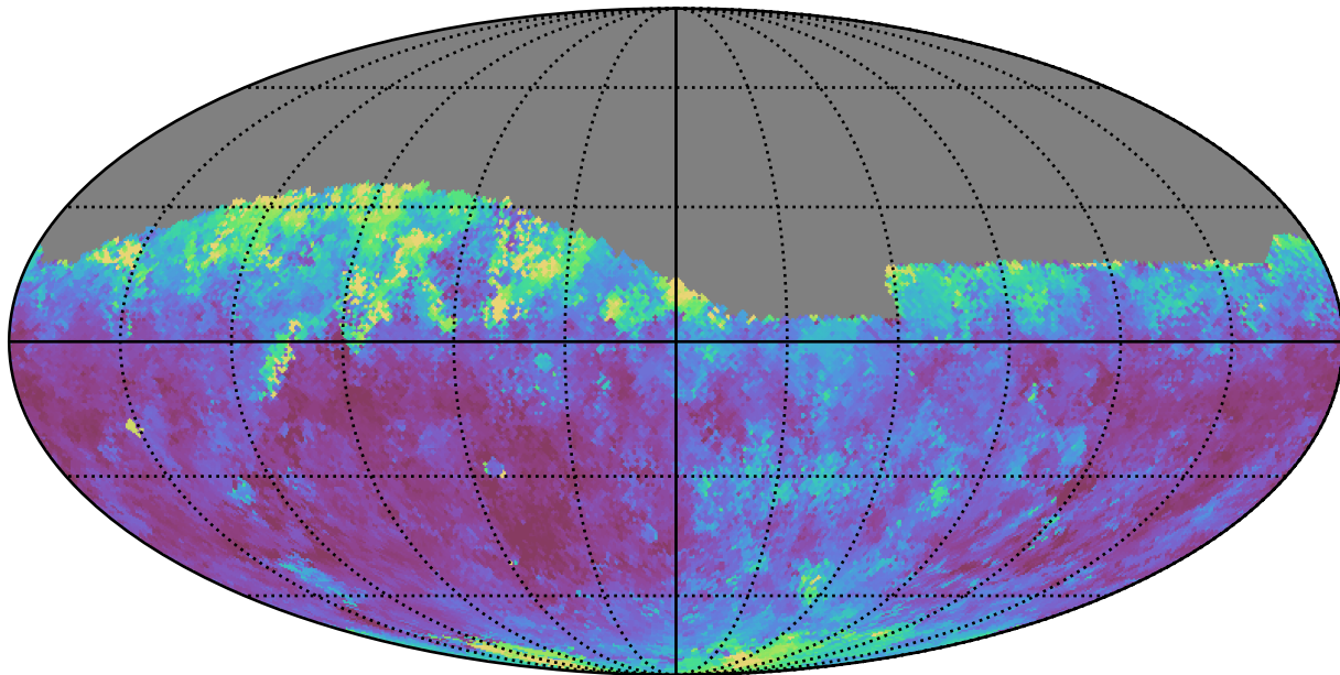
too_elab_r32_d2_giz_v3.4_10yrs Yr 1 i band: Median seeingEff
