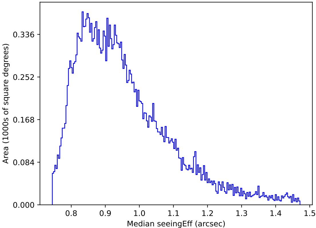
too_elab_r32_d2_giz_v3.4_10yrs Yr 1 i band: Median seeingEff
