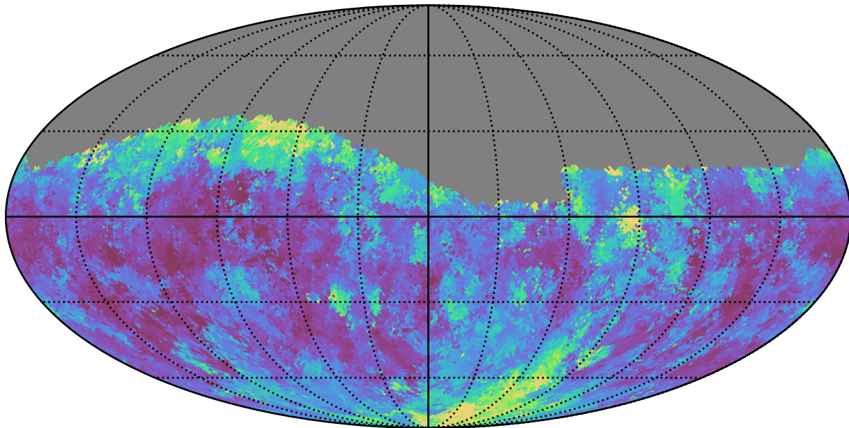
too_elab_r32_d2_giz_v3.4_10yrs Yr 1 g band: Median seeingEff
