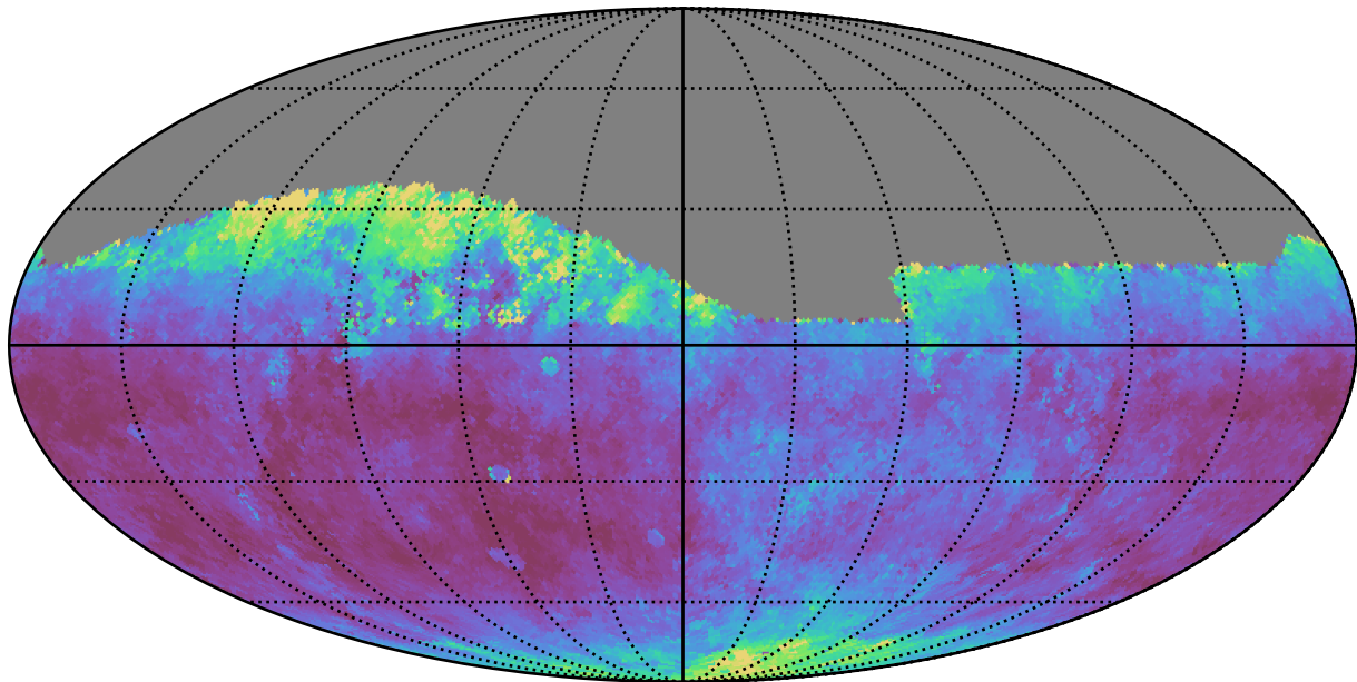
too_elab_r32_d2_giz_v3.4_10yrs Yr 1 all bands: Median seeingEff
