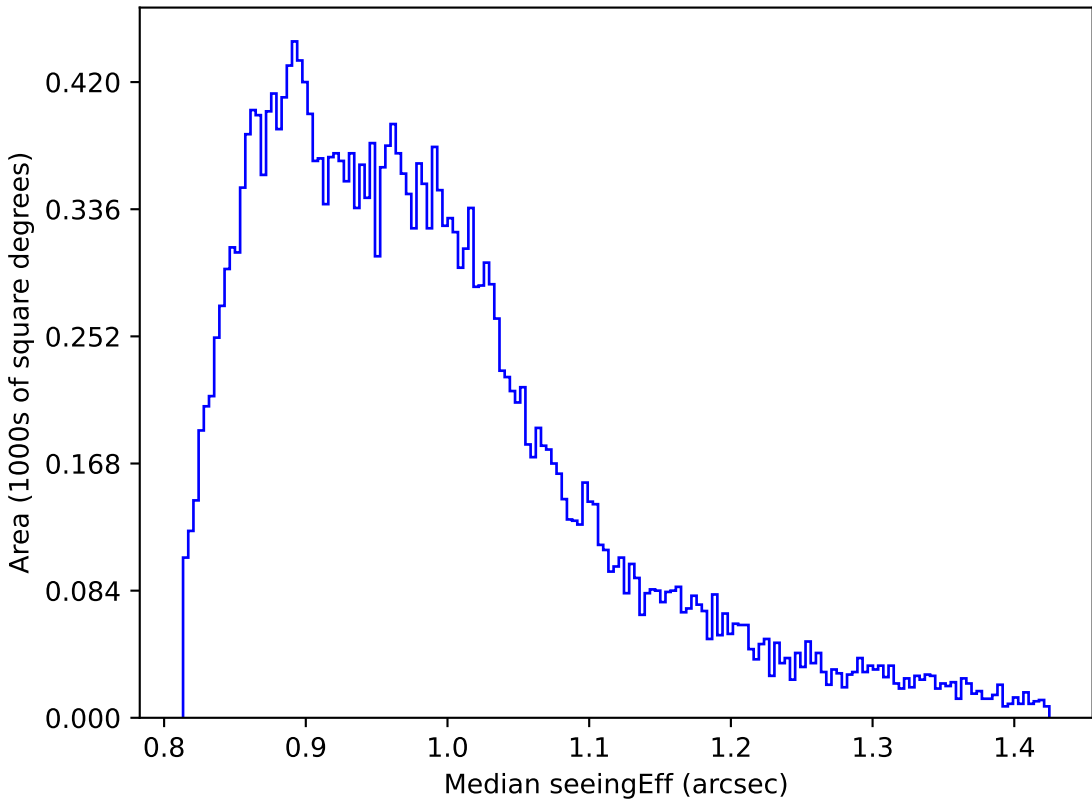
too_elab_r32_d2_giz_v3.4_10yrs Yr 1 all bands: Median seeingEff
