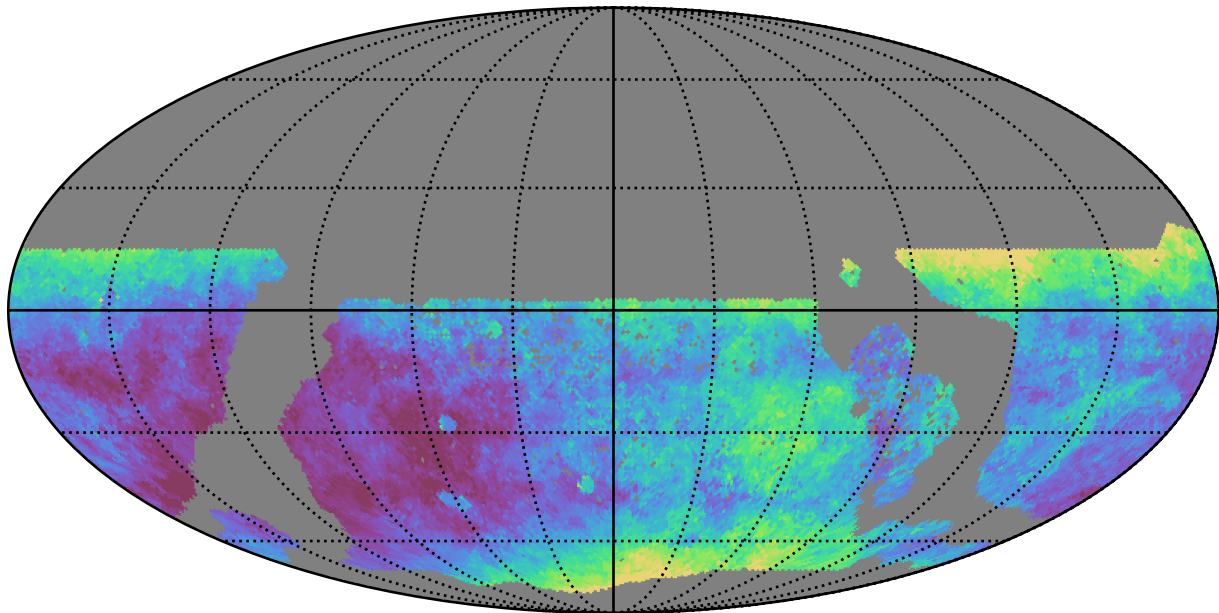
too_elab_r32_d2_giz_v3.4_10yrs WFD z band: Median seeingEff
