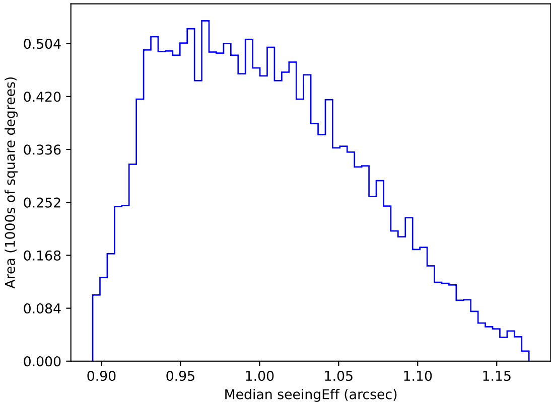
too_elab_r32_d2_giz_v3.4_10yrs WFD y band: Median seeingEff
