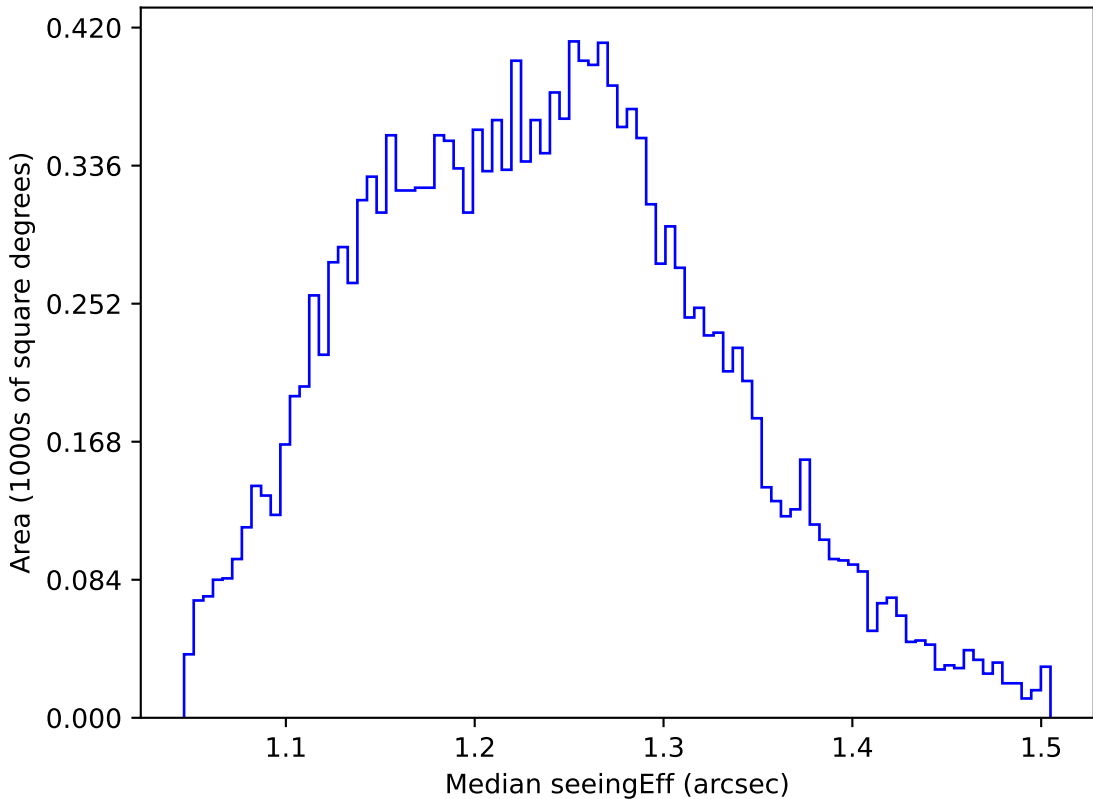
too_elab_r32_d2_giz_v3.4_10yrs WFD u band: Median seeingEff
