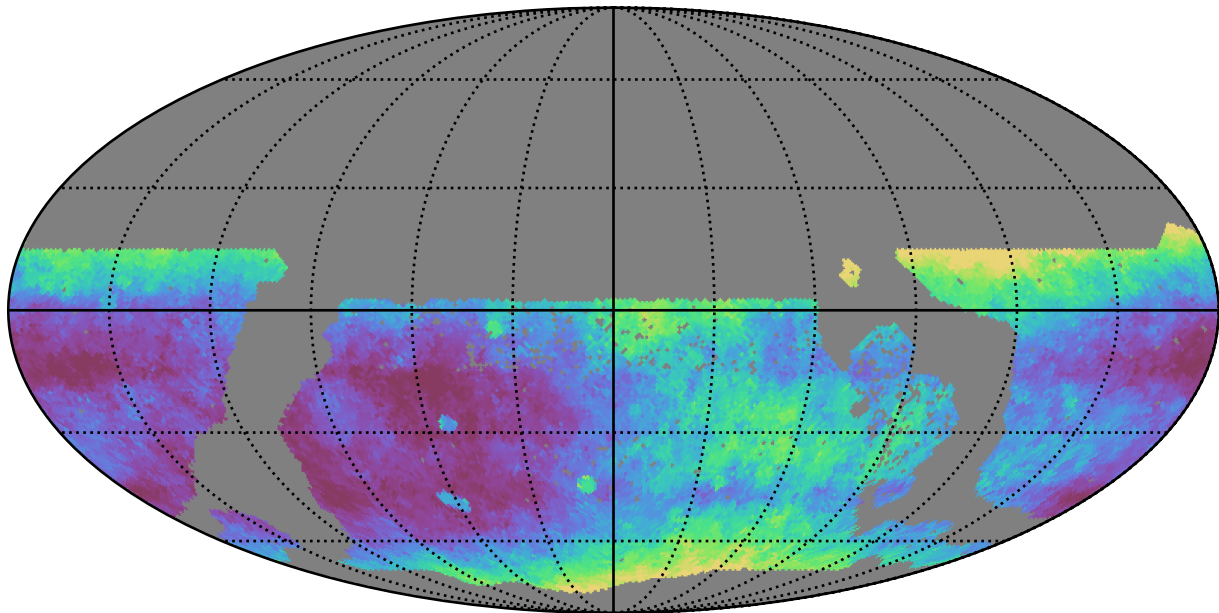
too_elab_r32_d2_giz_v3.4_10yrs WFD r band: Median seeingEff
