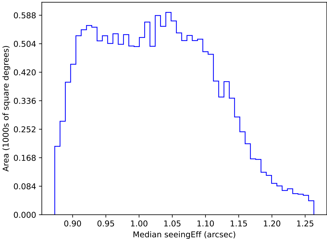
too_elab_r32_d2_giz_v3.4_10yrs WFD r band: Median seeingEff
