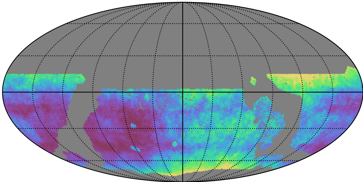
too_elab_r32_d2_giz_v3.4_10yrs WFD i band: Median seeingEff
