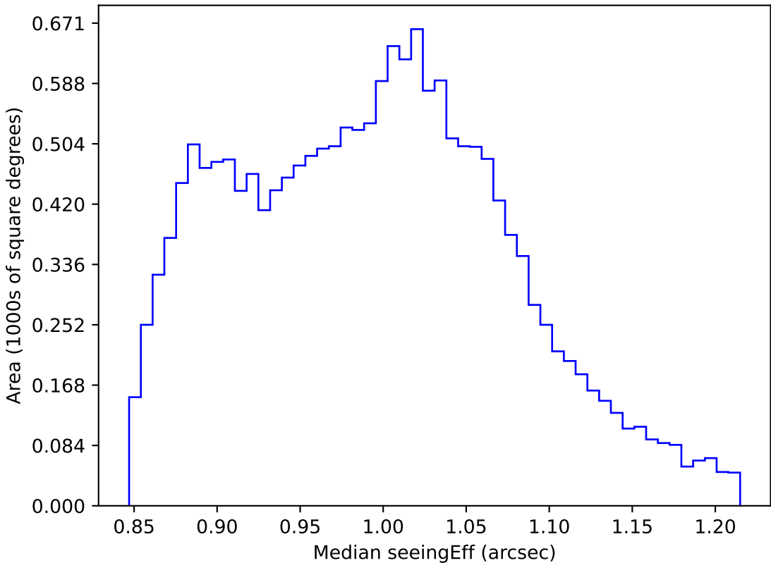
too_elab_r32_d2_giz_v3.4_10yrs WFD i band: Median seeingEff
