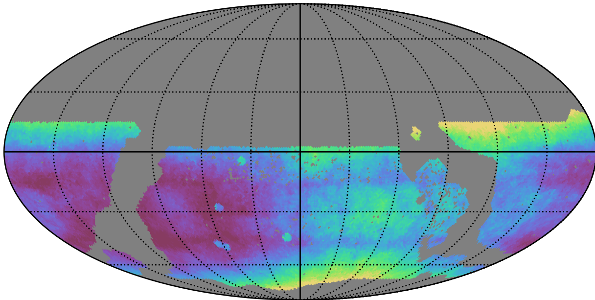
too_elab_r32_d2_giz_v3.4_10yrs WFD all bands: Median seeingEff
