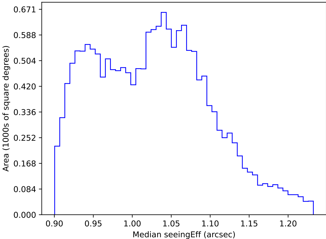
too_elab_r32_d2_giz_v3.4_10yrs WFD all bands: Median seeingEff
