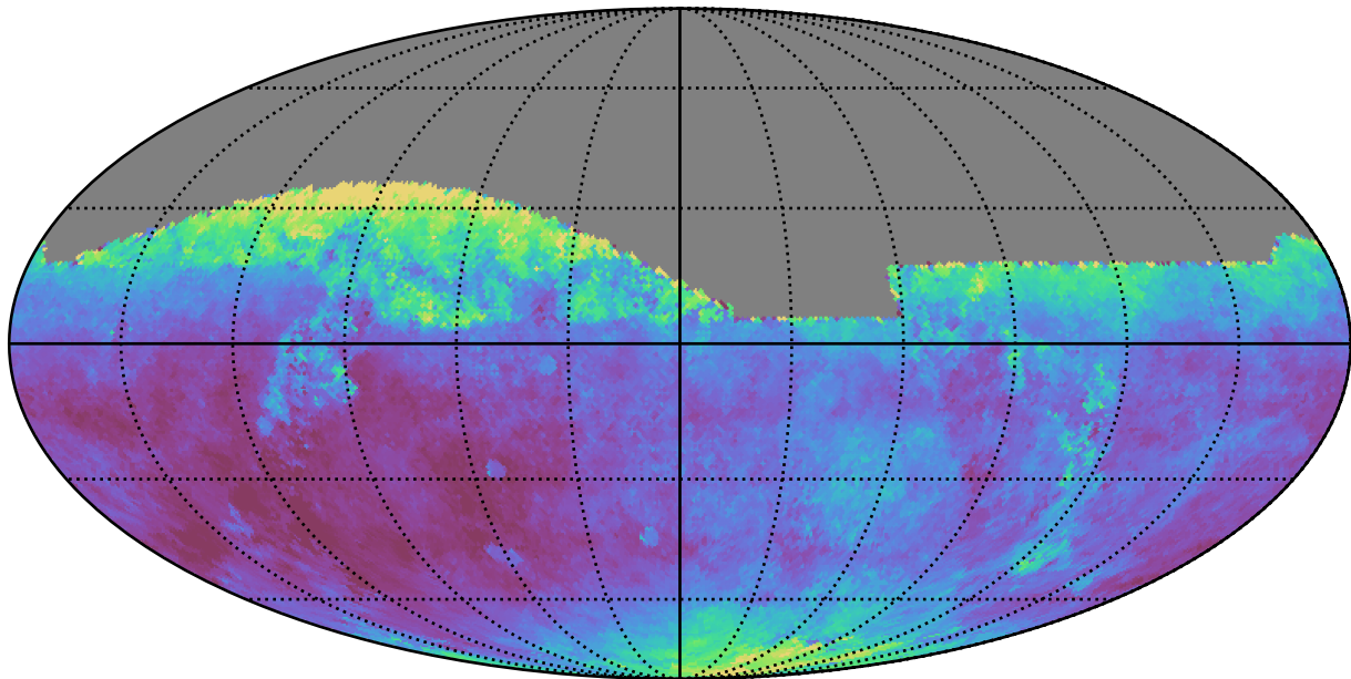
too_elab_r32_d2_giz_v3.4_10yrs All sky z band: Median seeingEff
