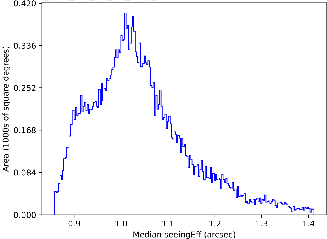
too_elab_r32_d2_giz_v3.4_10yrs All sky z band: Median seeingEff
