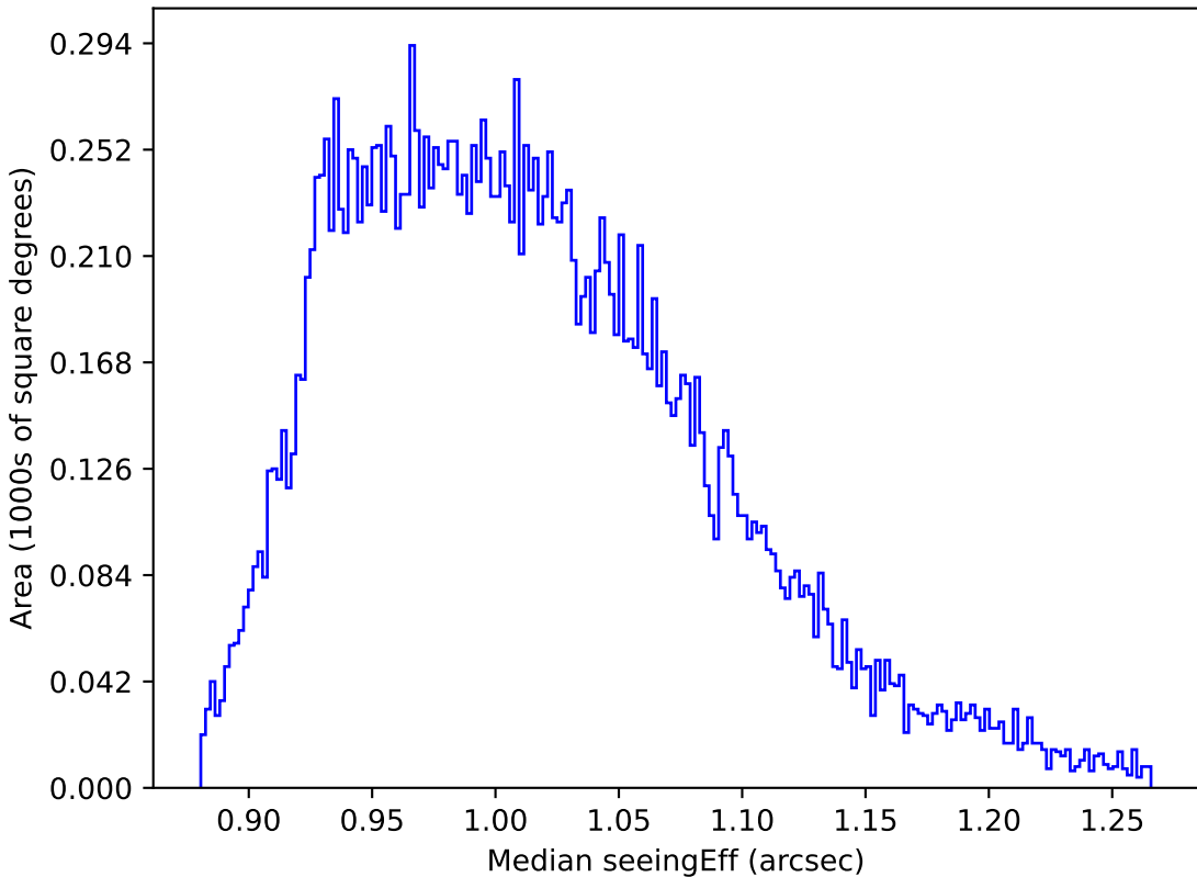
too_elab_r32_d2_giz_v3.4_10yrs All sky y band: Median seeingEff
