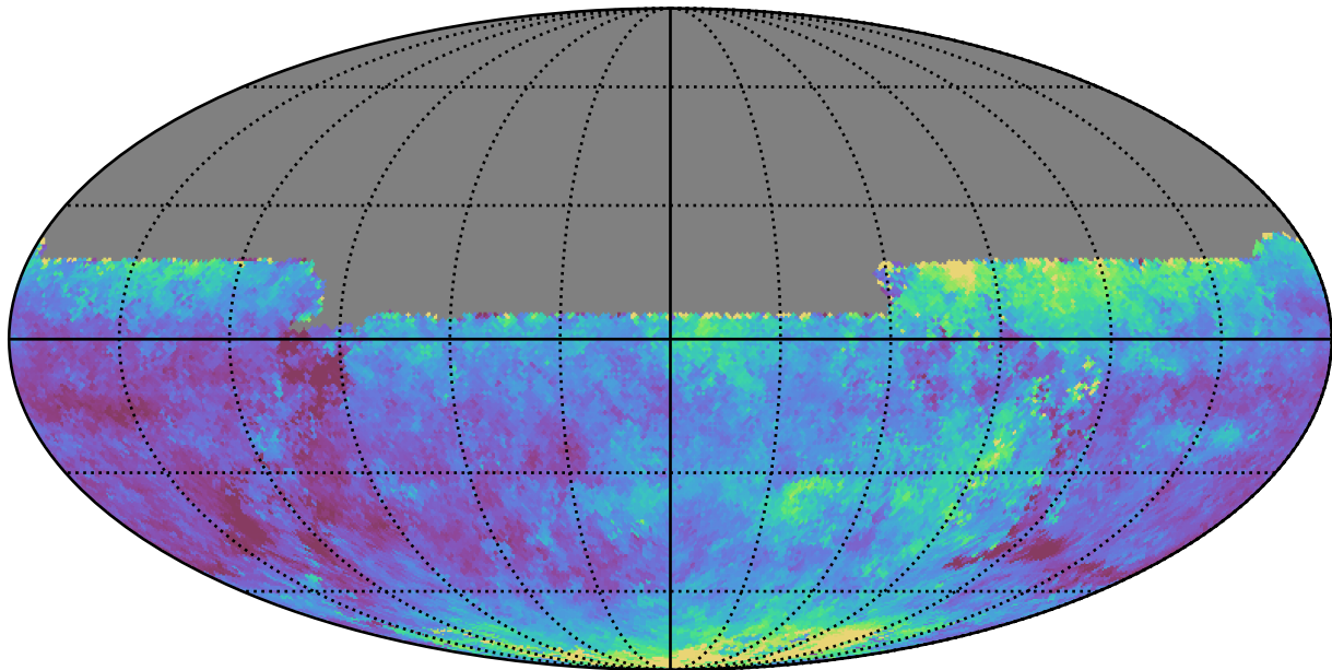
too_elab_r32_d2_giz_v3.4_10yrs All sky u band: Median seeingEff
