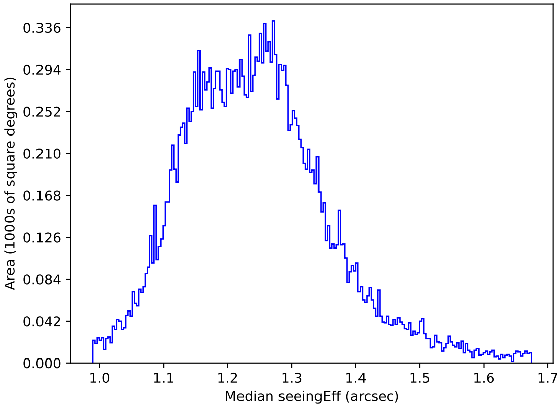
too_elab_r32_d2_giz_v3.4_10yrs All sky u band: Median seeingEff
