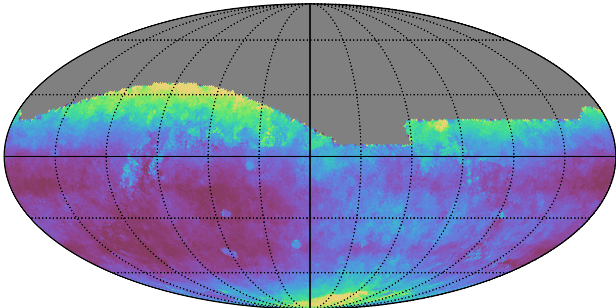
too_elab_r32_d2_giz_v3.4_10yrs All sky r band: Median seeingEff
