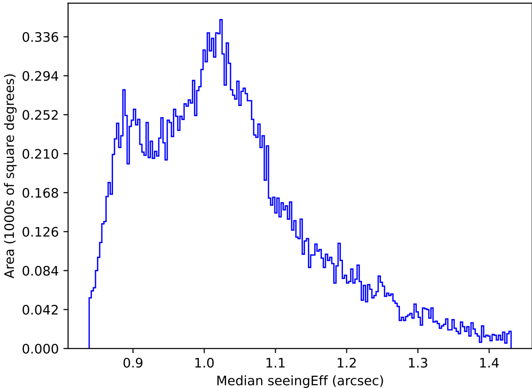
too_elab_r32_d2_giz_v3.4_10yrs All sky i band: Median seeingEff
