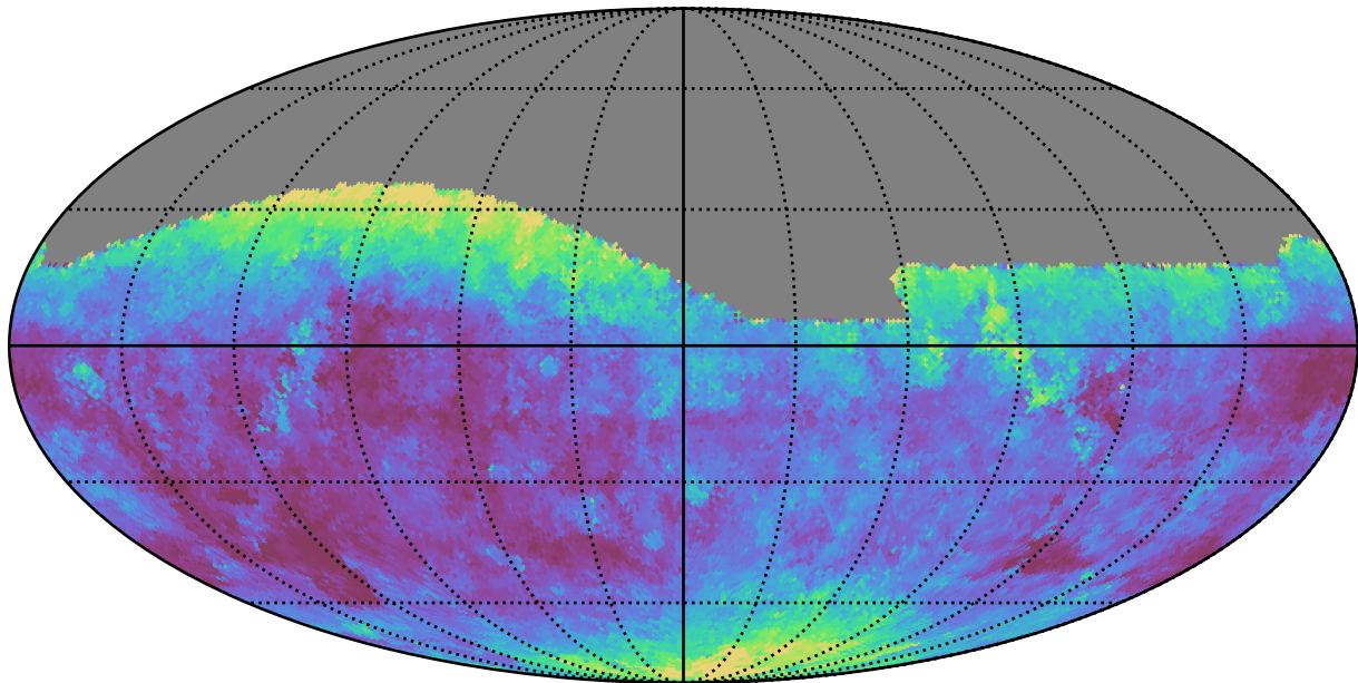
too_elab_r32_d2_giz_v3.4_10yrs All sky g band: Median seeingEff
