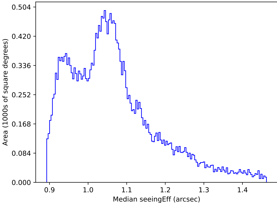
too_elab_r32_d2_giz_v3.4_10yrs All sky all bands: Median seeingEff
