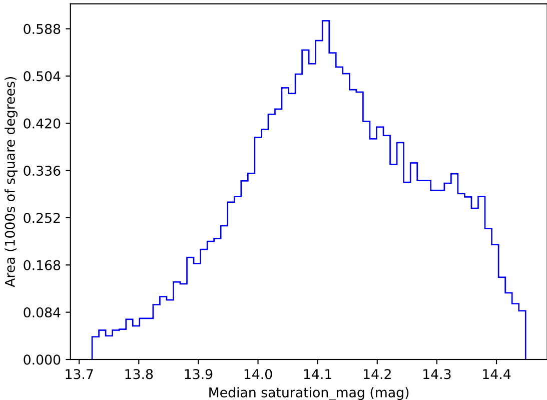
too_elab_r32_d2_giz_v3.4_10yrs WFD z band: Median saturation_mag
