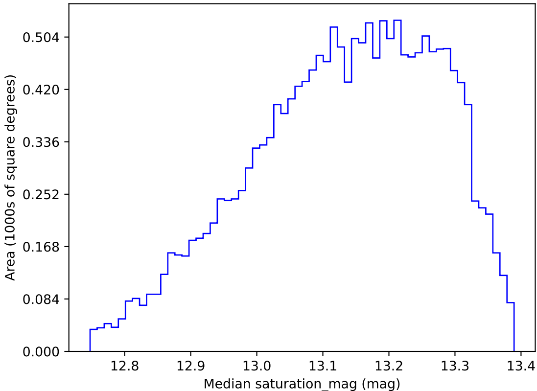
too_elab_r32_d2_giz_v3.4_10yrs WFD y band: Median saturation_mag
