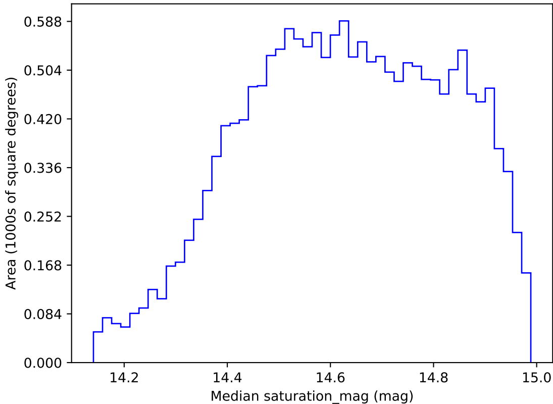
too_elab_r32_d2_giz_v3.4_10yrs WFD r band: Median saturation_mag
