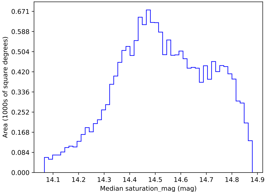
too_elab_r32_d2_giz_v3.4_10yrs WFD i band: Median saturation_mag
