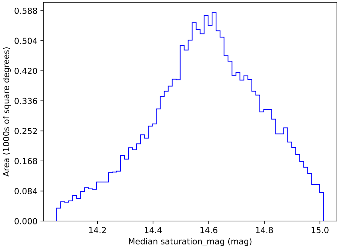
too_elab_r32_d2_giz_v3.4_10yrs WFD g band: Median saturation_mag
