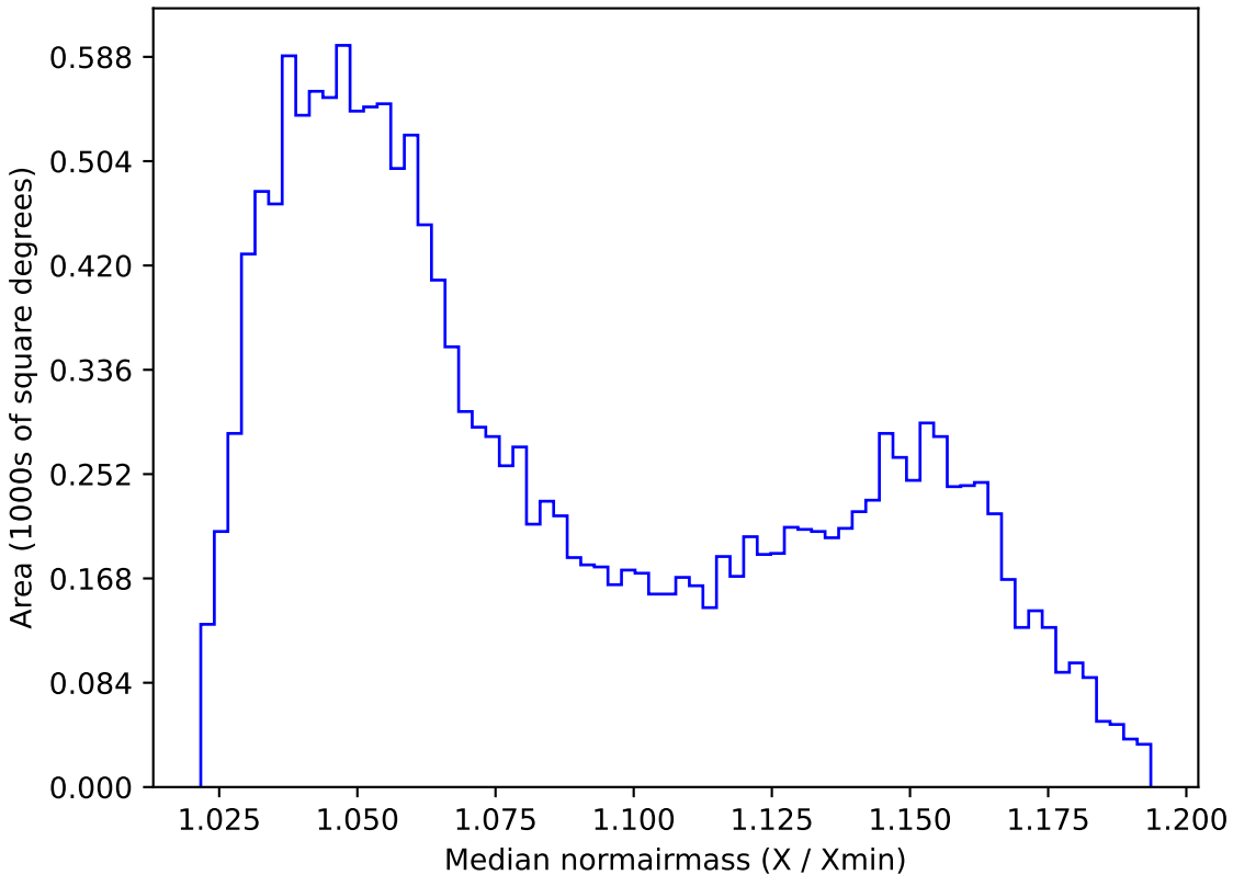
too_elab_r32_d2_giz_v3.4_10yrs WFD z band: Median normairmass
